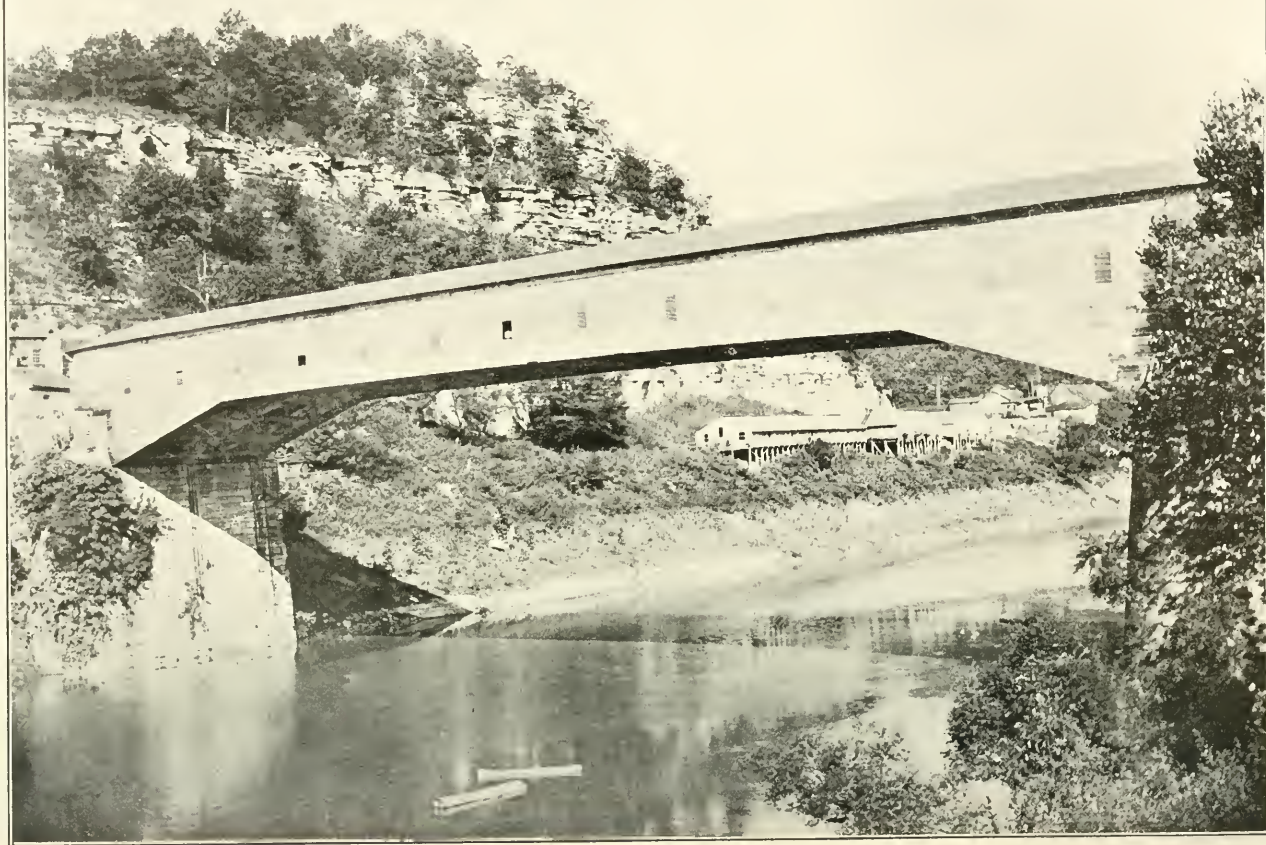
WOODEN BRIDGE OVER KENTUCKY RIVER, AT MOUTH OF HICKMAN CREEK.
