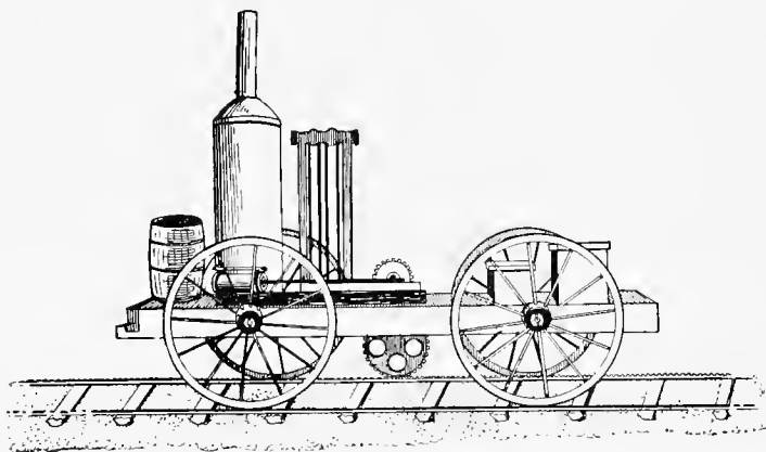
MODEL OF THE JOHN STEVENS LOCOMOTIVE. THE FIRST IN AMERICA. 1825
