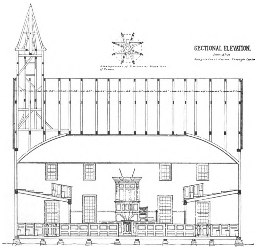
One of Louis Rue's Drawings of Old Tennent Church.
