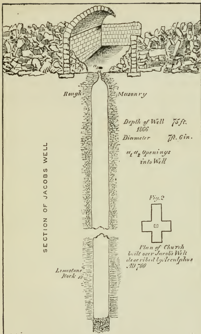
RUINED CRYPT, AND SECTION OF JACOB'S WELL
