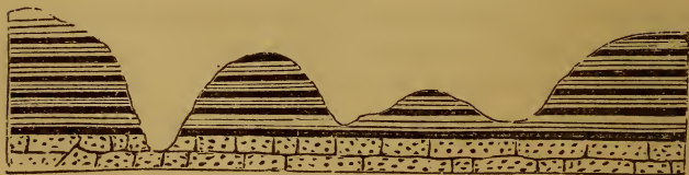
FIG. 7.—Illinois Coal-Field (after Daddow).
