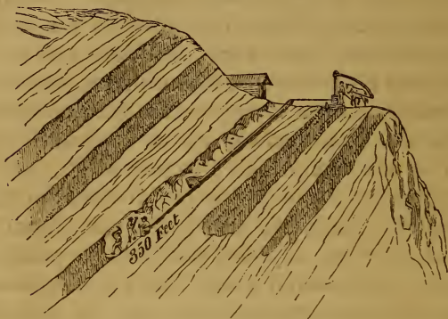
FIG. 10.—Section of Graphite Mine at Ticonderoga, New York.
