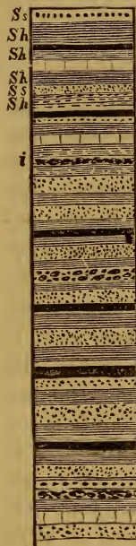
FIG. 4.—Ideal Section showing Alternation of Different Kinds of Strata. Ss , sandstone; Sh , shale; L , limestone; i , iron; and c , coal.
