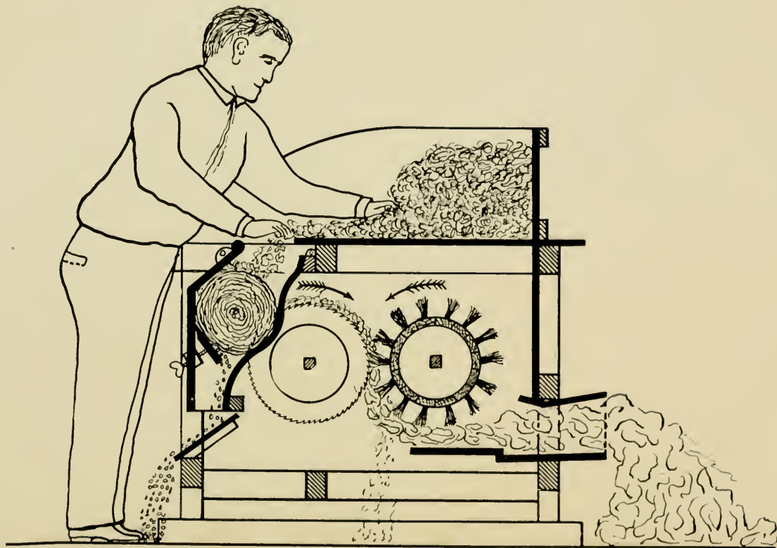
HOLMES' SAW GIN.
